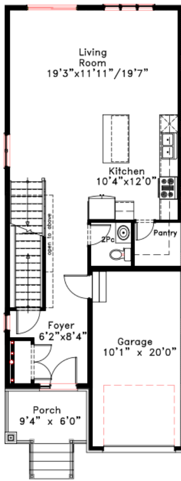
MAIN FLOOR
