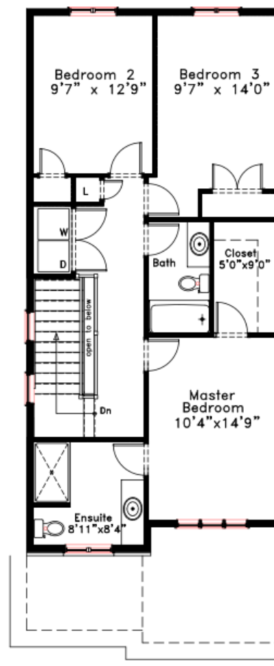
SECOND FLOOR
